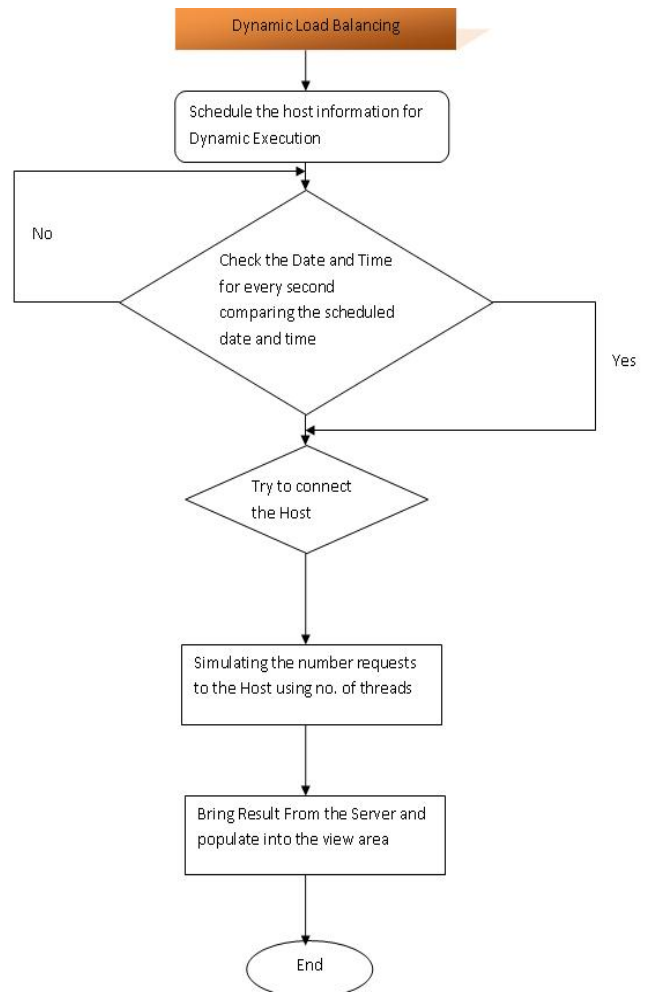
Fig. 5: Flow Chart of Dynamic load balancing Algorithm
