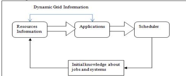
Fig. 2 Dynamic Load Balancing
