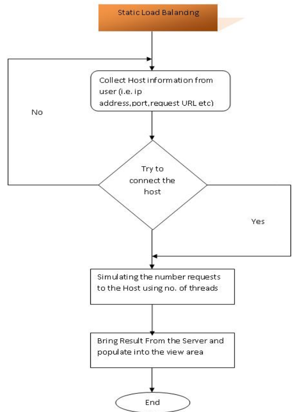
Fig. 4: Flow Chart of Static load balancing Algorithm
